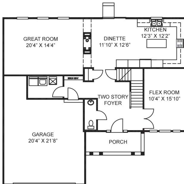
FIRST FLOOR: 1,132 SQ. FT.
