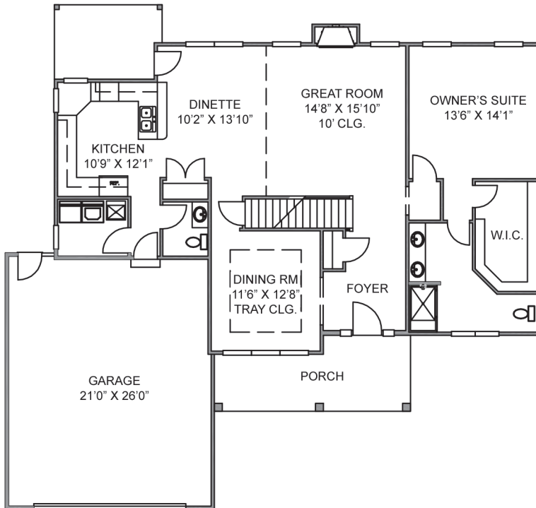
FIRST FLOOR: 1,407 SQ. FT.
