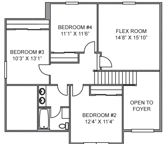
SECOND FLOOR: 848 SQ. FT.
