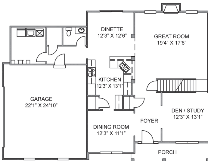
FIRST FLOOR: 1,407 SQ. FT.
